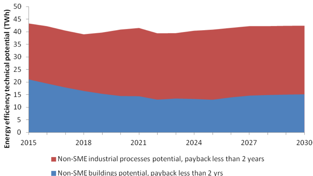
Figure 1: Projected technical potential for energy efficiency within scope of ESOS
