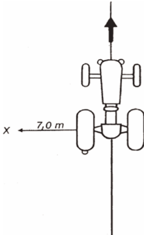
Figure 2 Measuring positions for stationary agricultural and forestry vehicles
