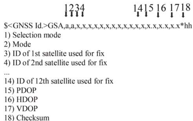
Figure 3 Structure of the GSA sentence
