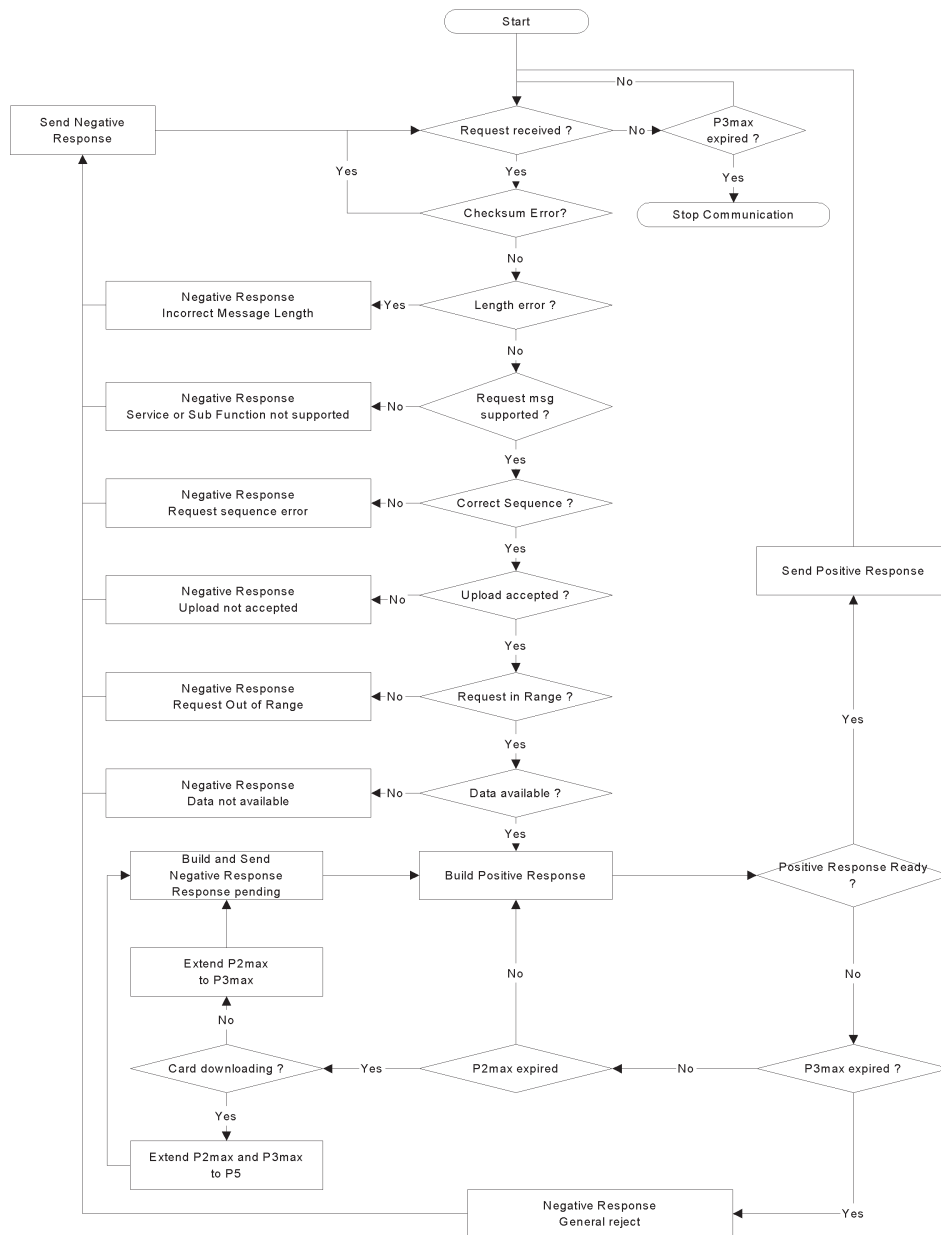
Figure 2 VU error handling
