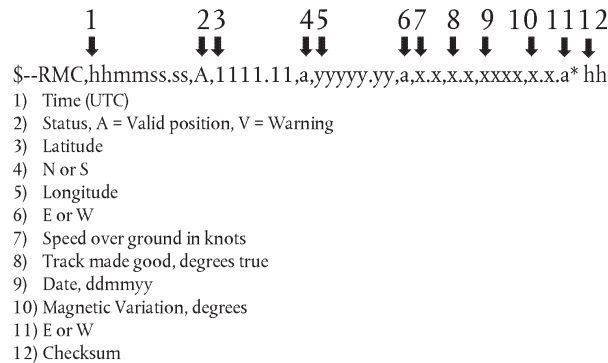
Figure 2 Structure of the RMC sentence
