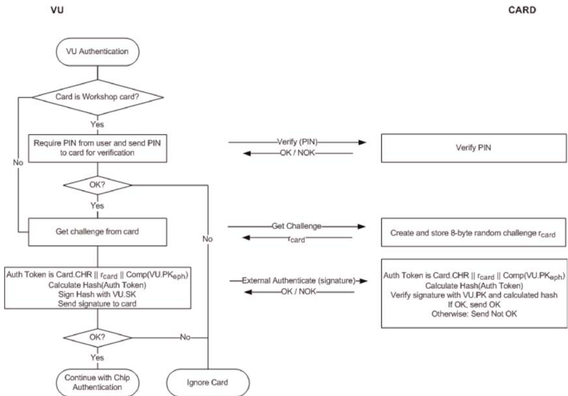
Figure 6 VU Authentication protocol
