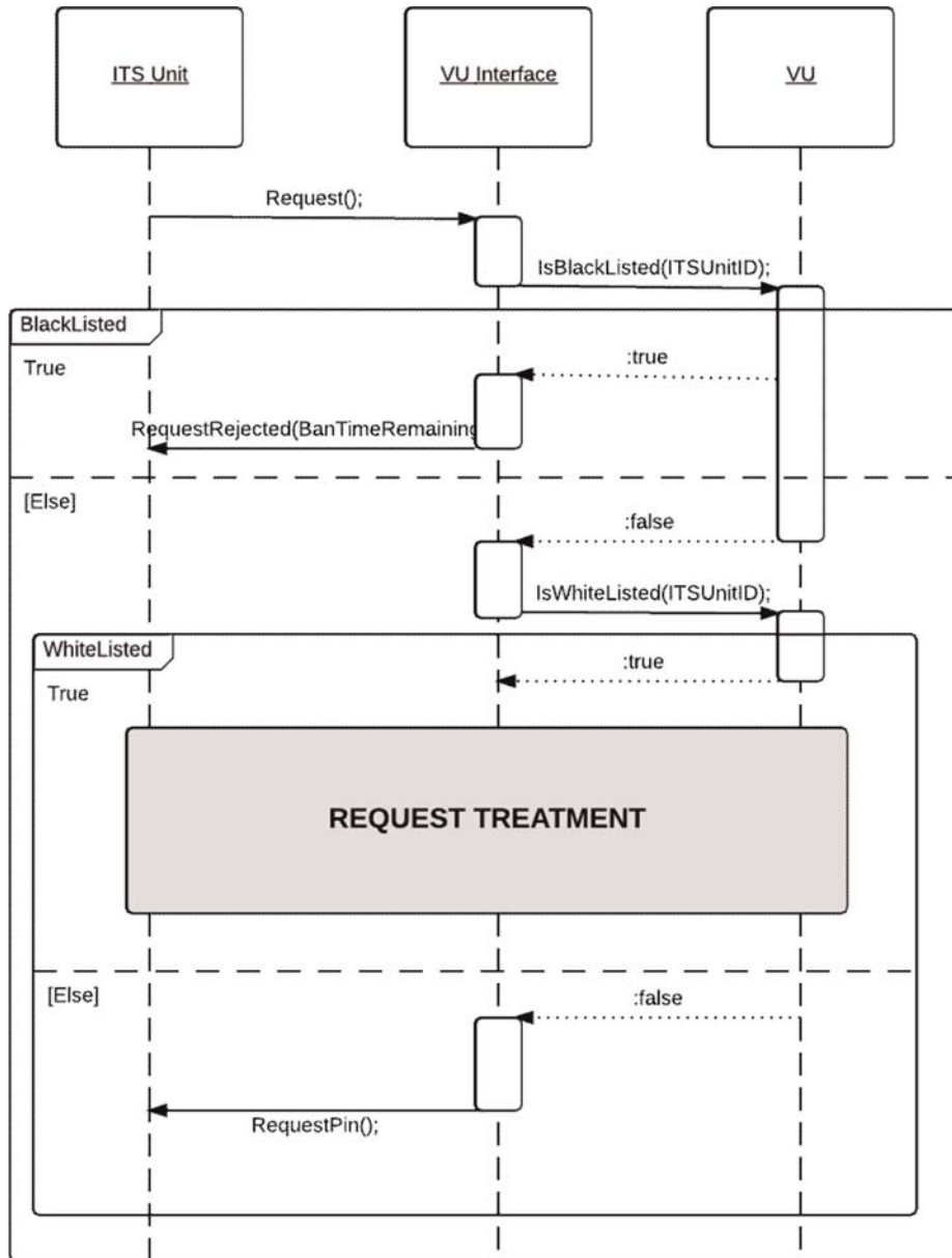
Sequence Diagram for ITS Unit's authorization verification
