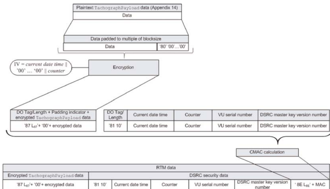
Tachograph payload encryption and MAC generation
