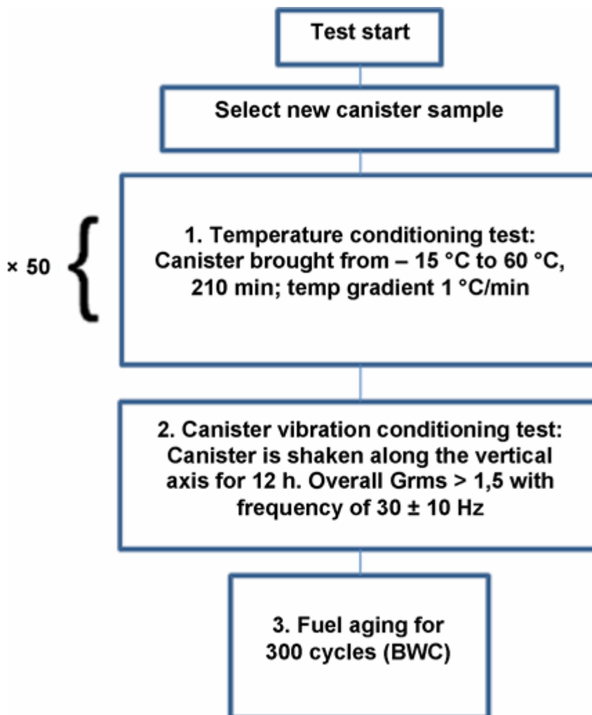
Figure 2 Canister bench aging procedure
