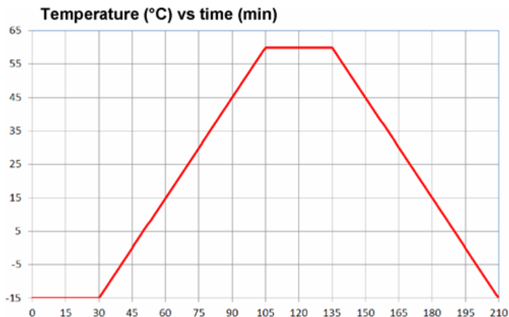
Figure 3 Temperature conditioning cycle
