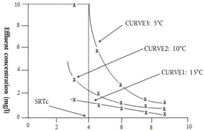
Figure 2 Regression Line SRT · S1 vs S1 at T = 5 °C
