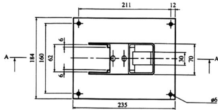
Figure 2 Support stand
