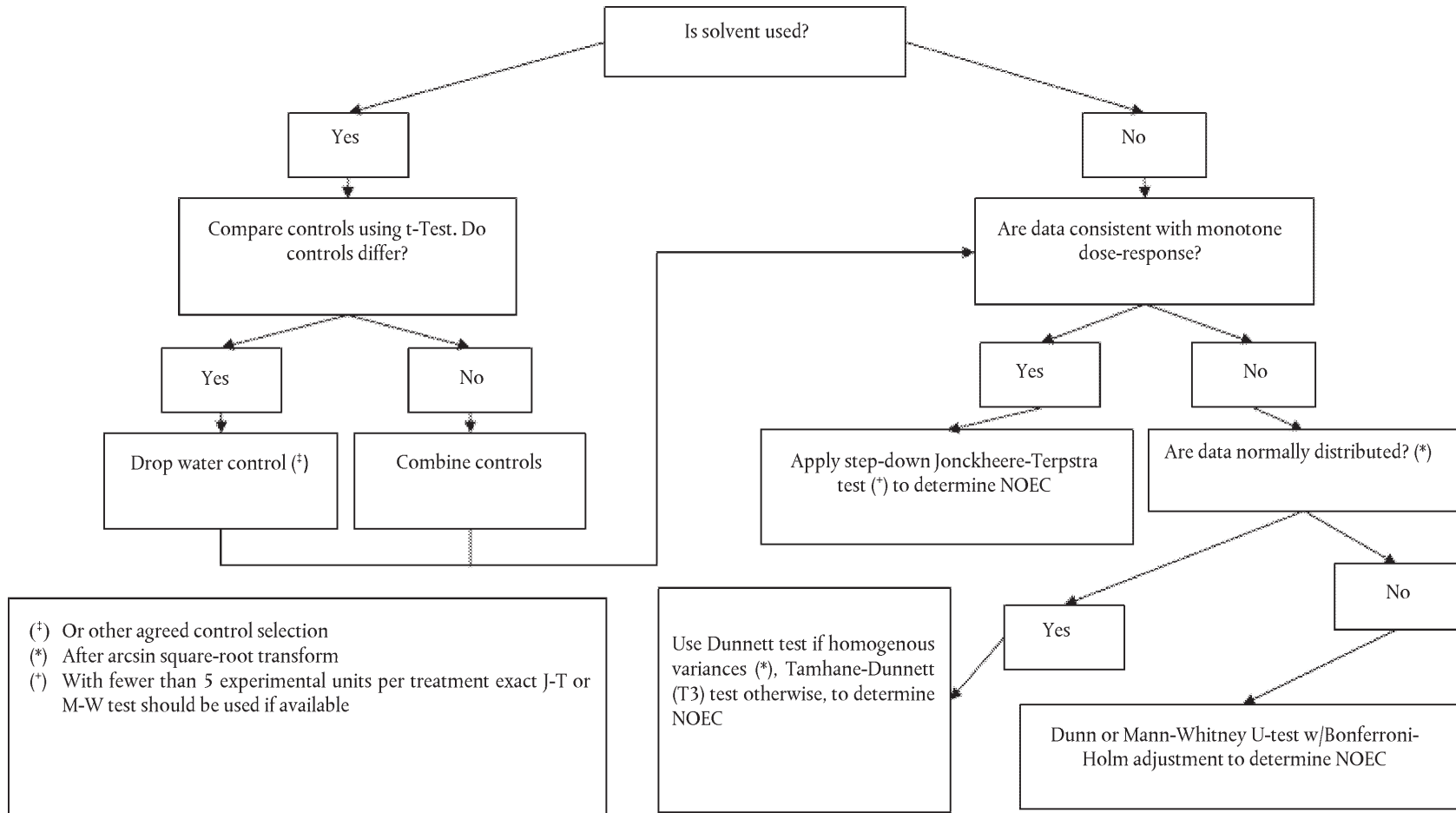
Statistical Flow Chart for sex ratio analysis
