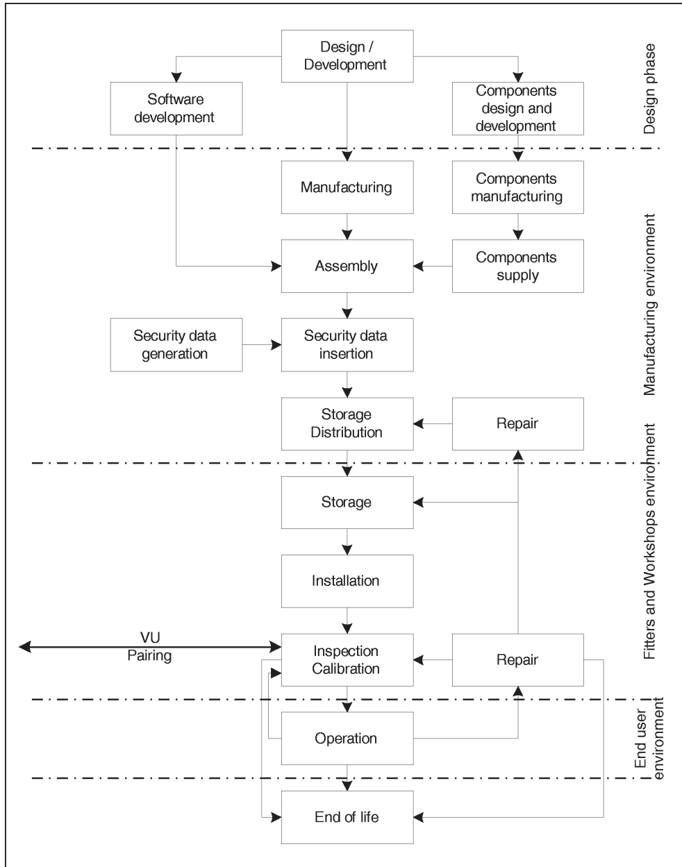
Figure 2 Motion sensor typical life cycle
