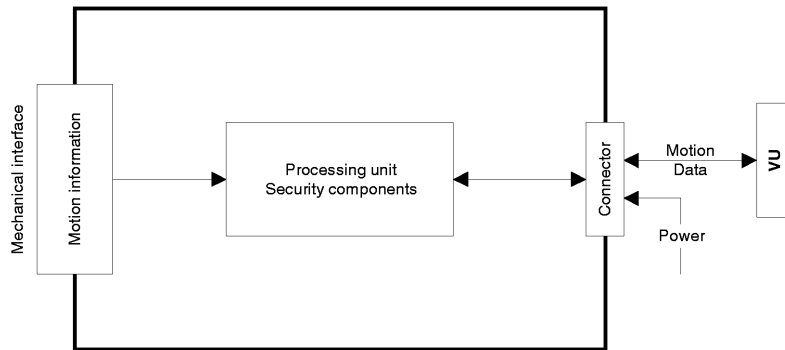
Figure 1 Typical motion sensor
