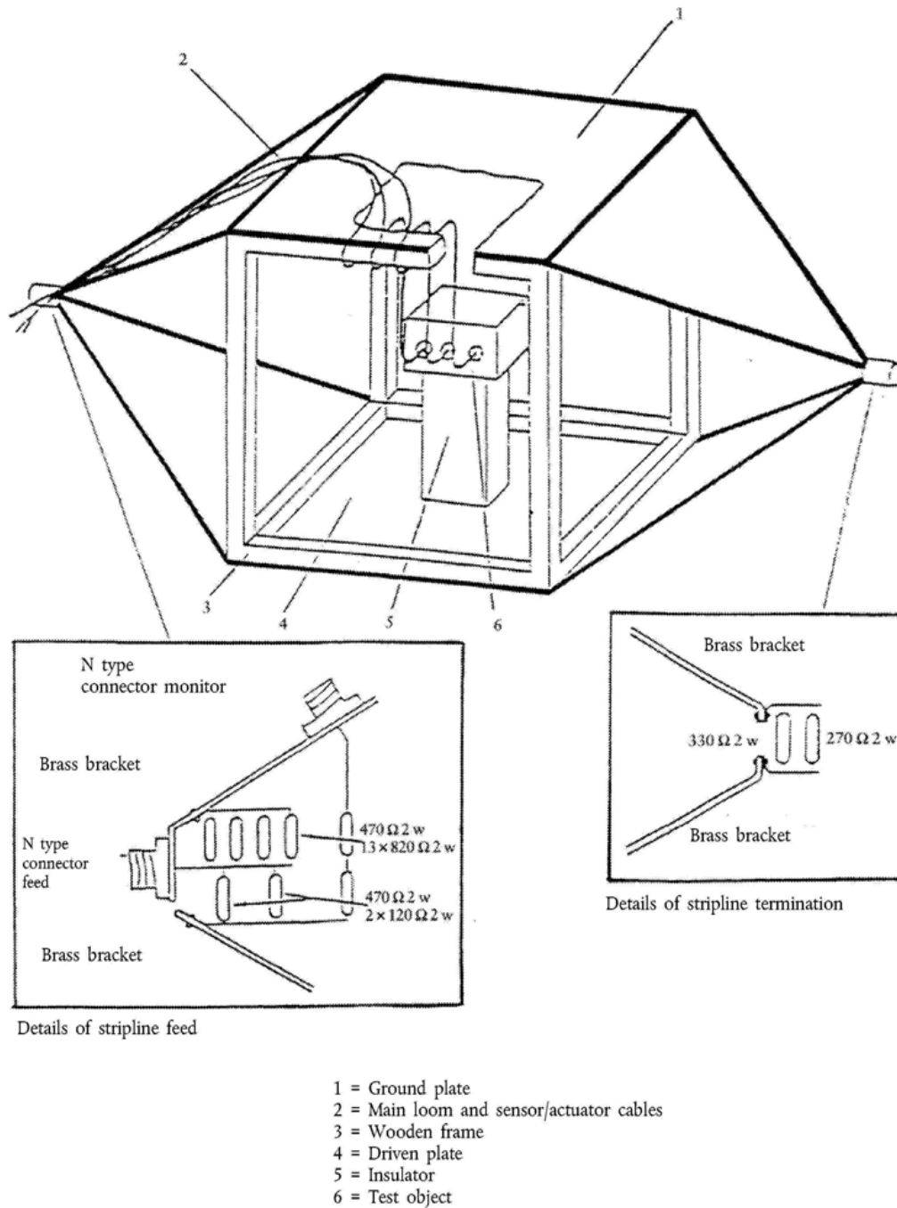
Figure 2 800 mm stripline dimensions
