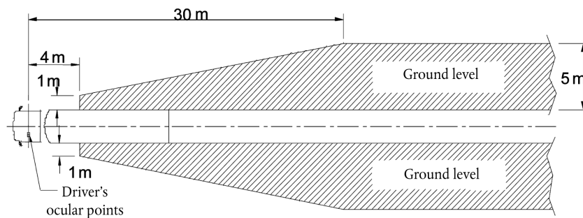
Figure 7: Field of vision of Class II mirrors
