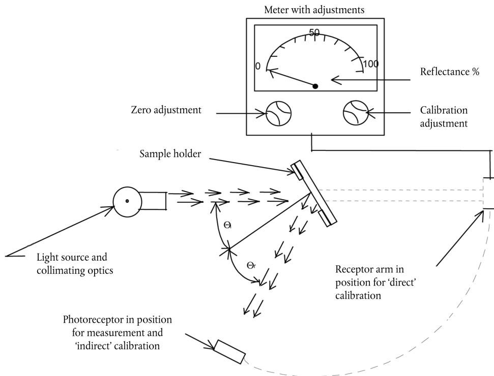
Figure 4: Generalised reflectometer showing experimental set-ups for the two calibration methods
