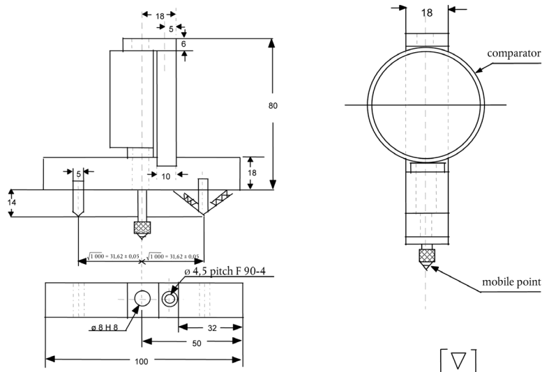
Figure 3: spherometer
