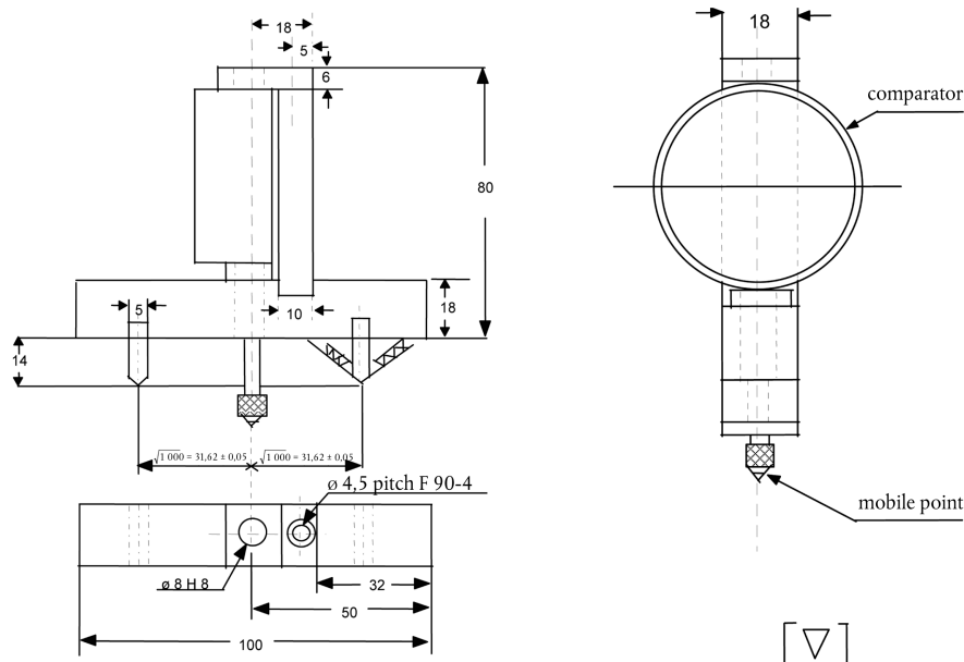
Figure 3: spherometer
