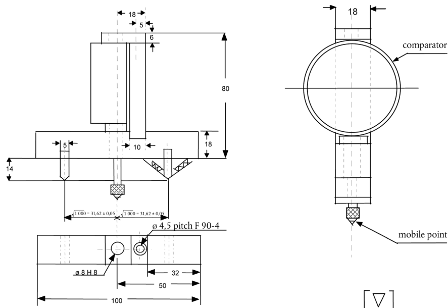
Figure 3: spherometer
