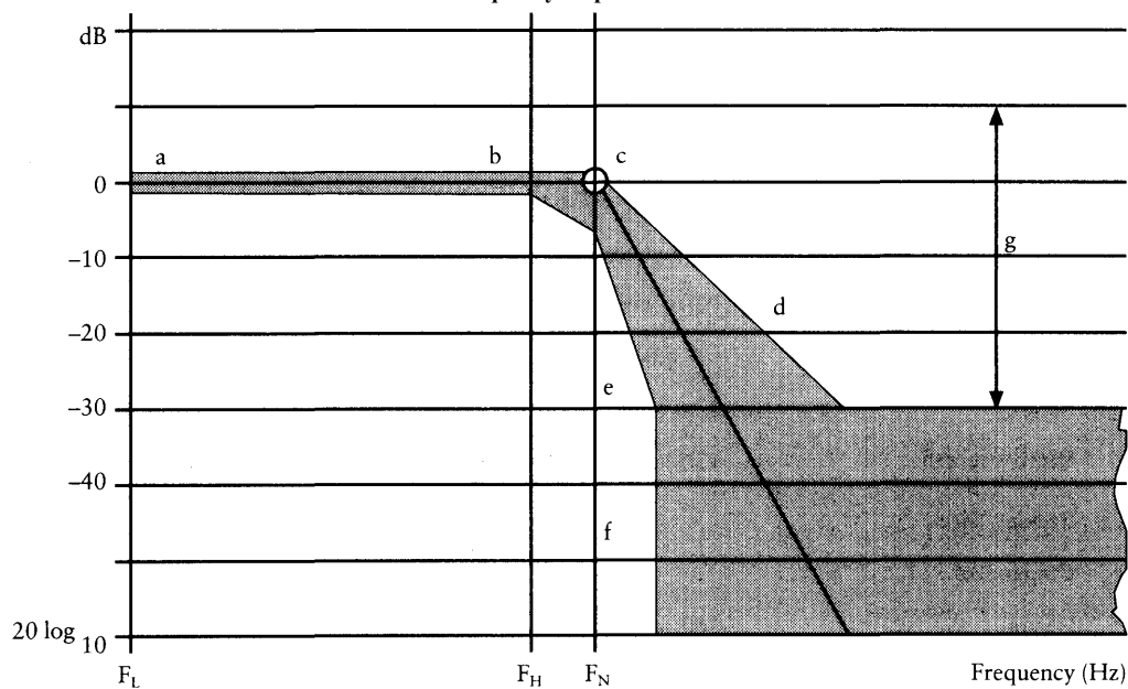
Figure 1 Frequency response curve
