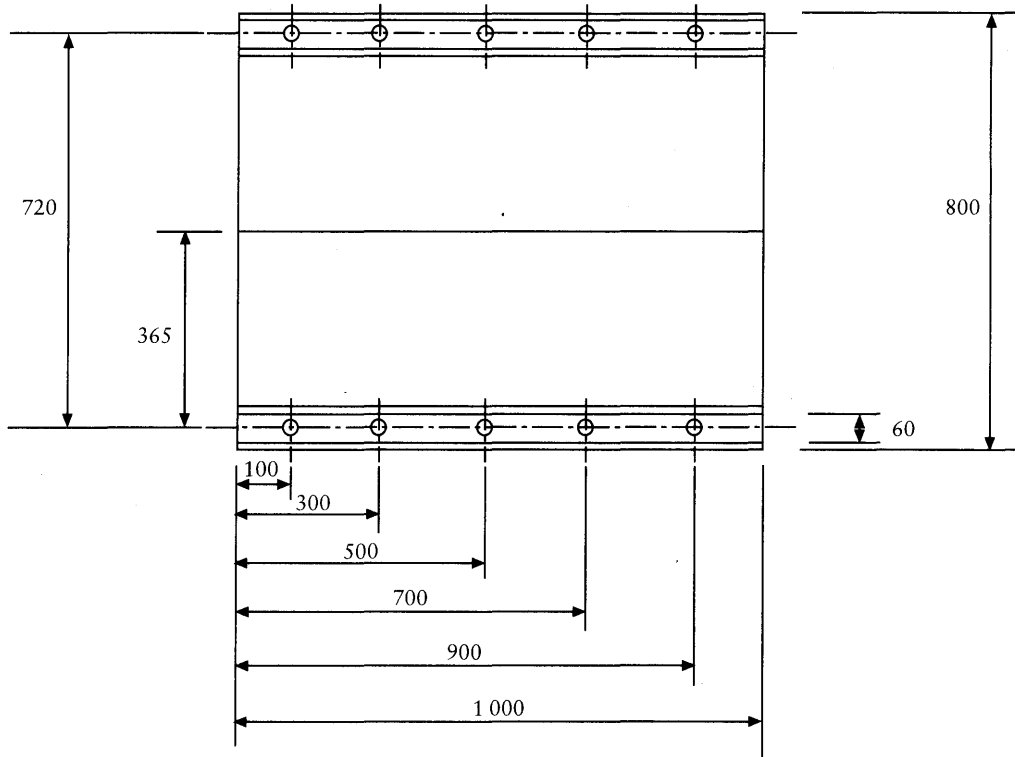
Figure 5 Positions of holes for barrier mounting
