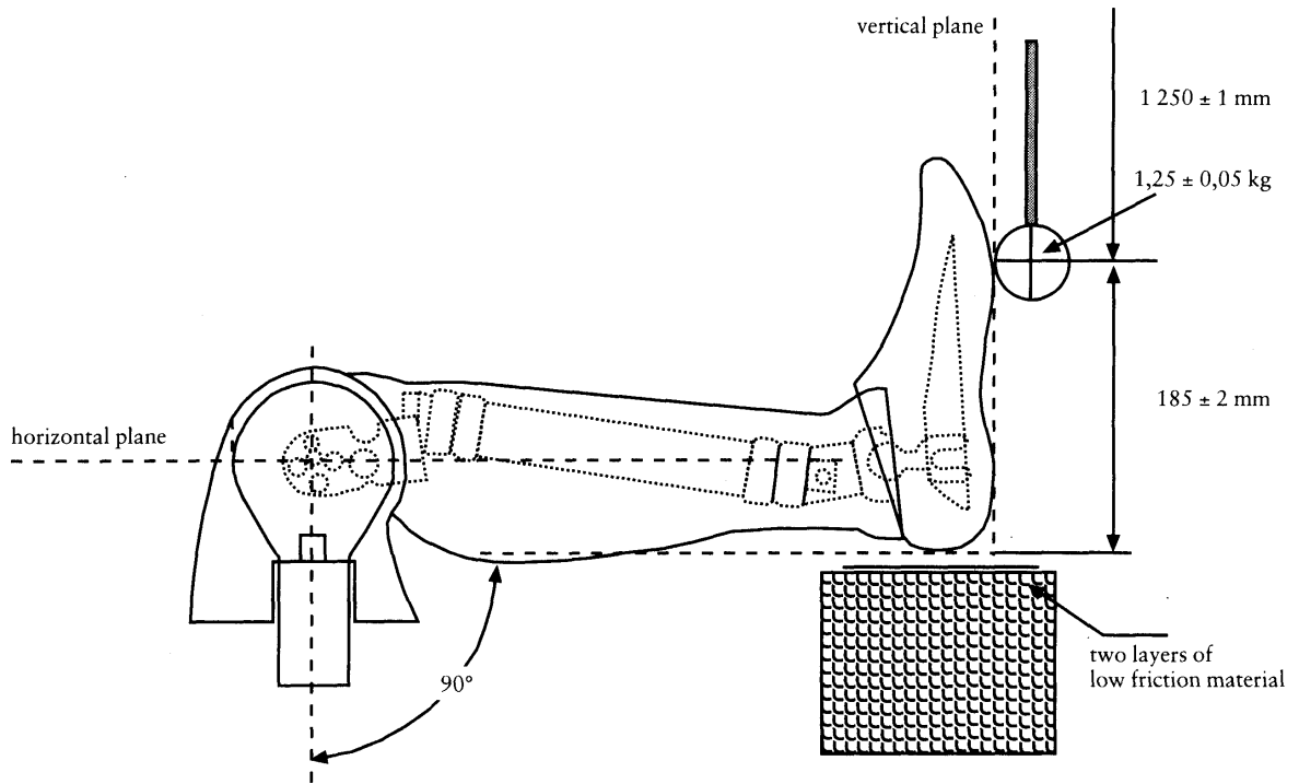
Figure 1a Upper foot impact test — test set-up specifications
