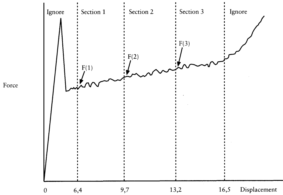
Figure 4 Crush force and displacement
