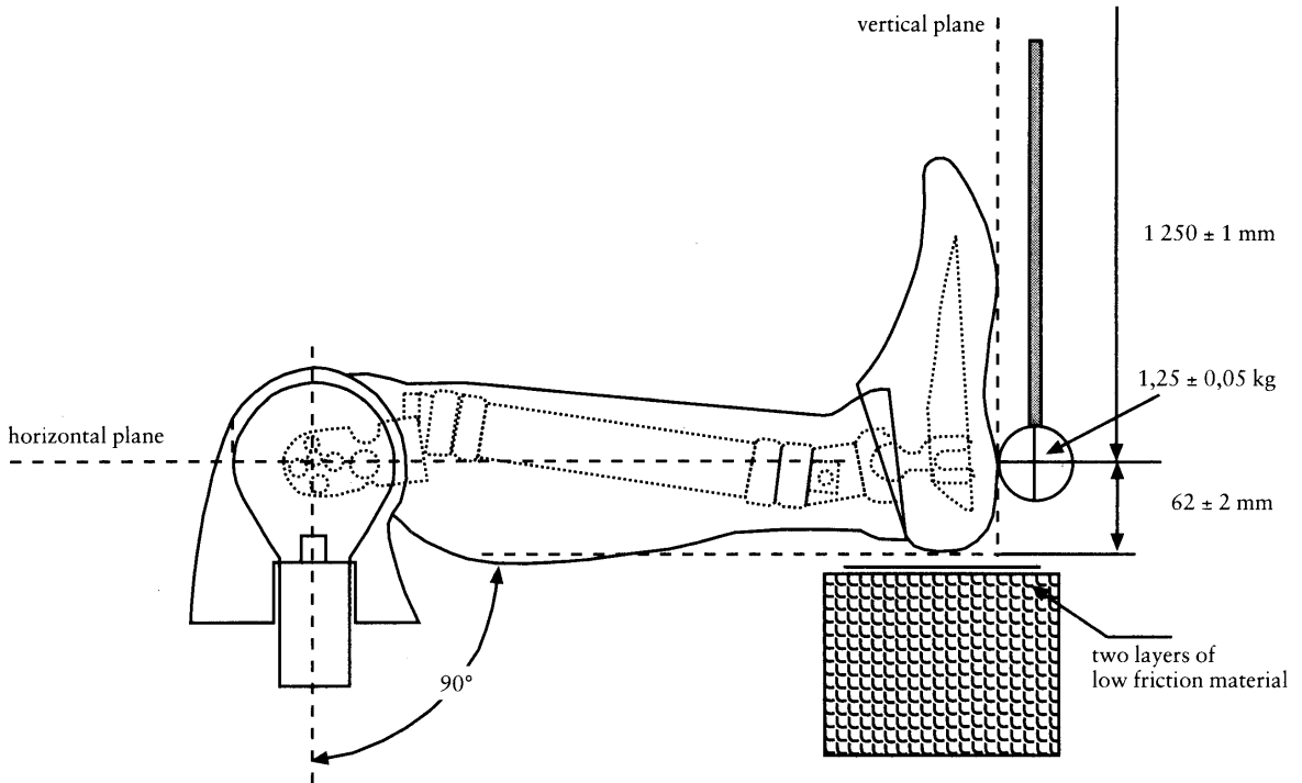
Figure 1b Lower foot impact test — test set-up specifications
