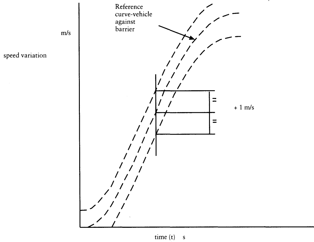
Figure 1 Equivalence curve — tolerance band for curve V = f(t)
