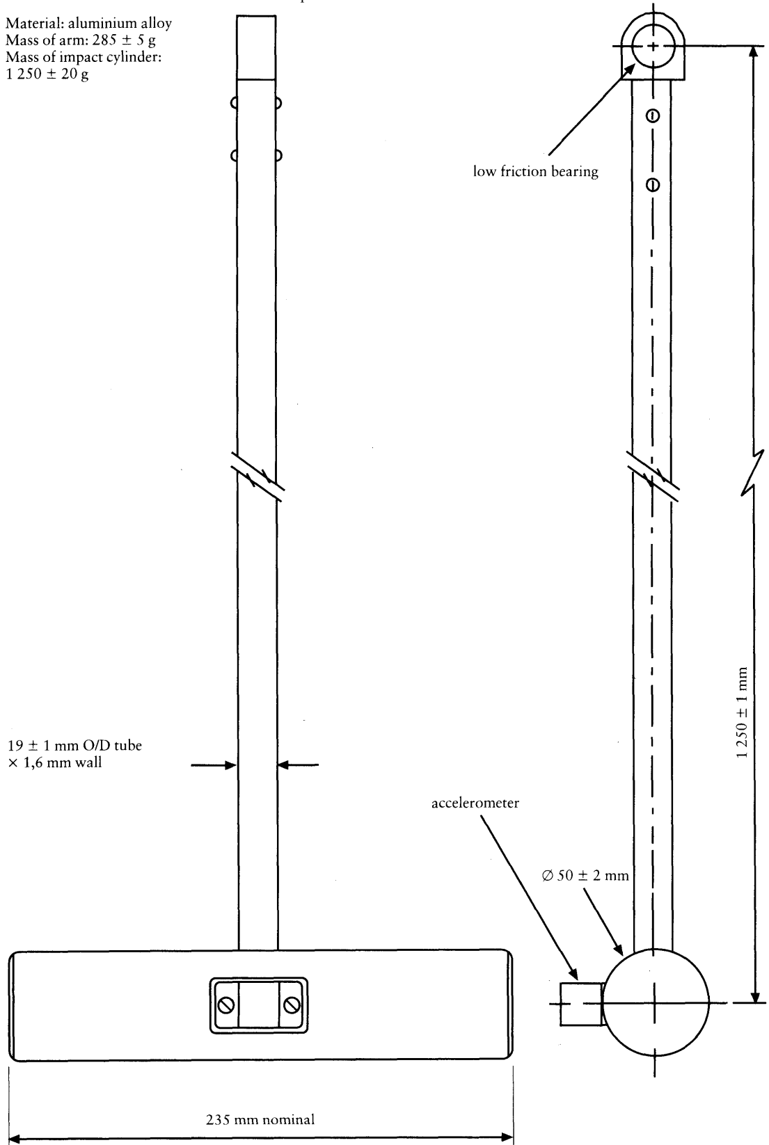
Figure 3a Pendulum impactor
