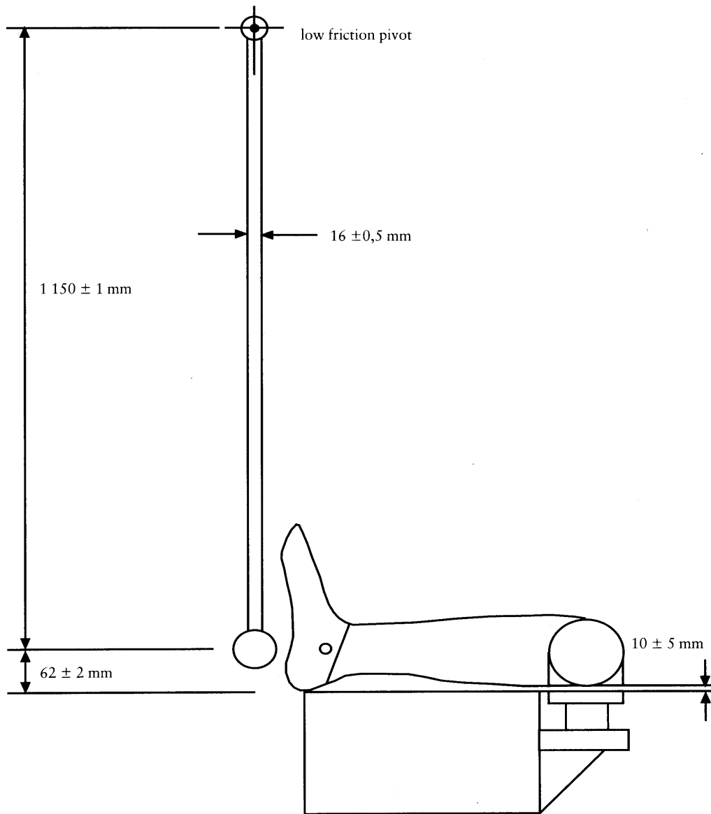
Figure 3 Lower foot impact test — test set-up specifications
