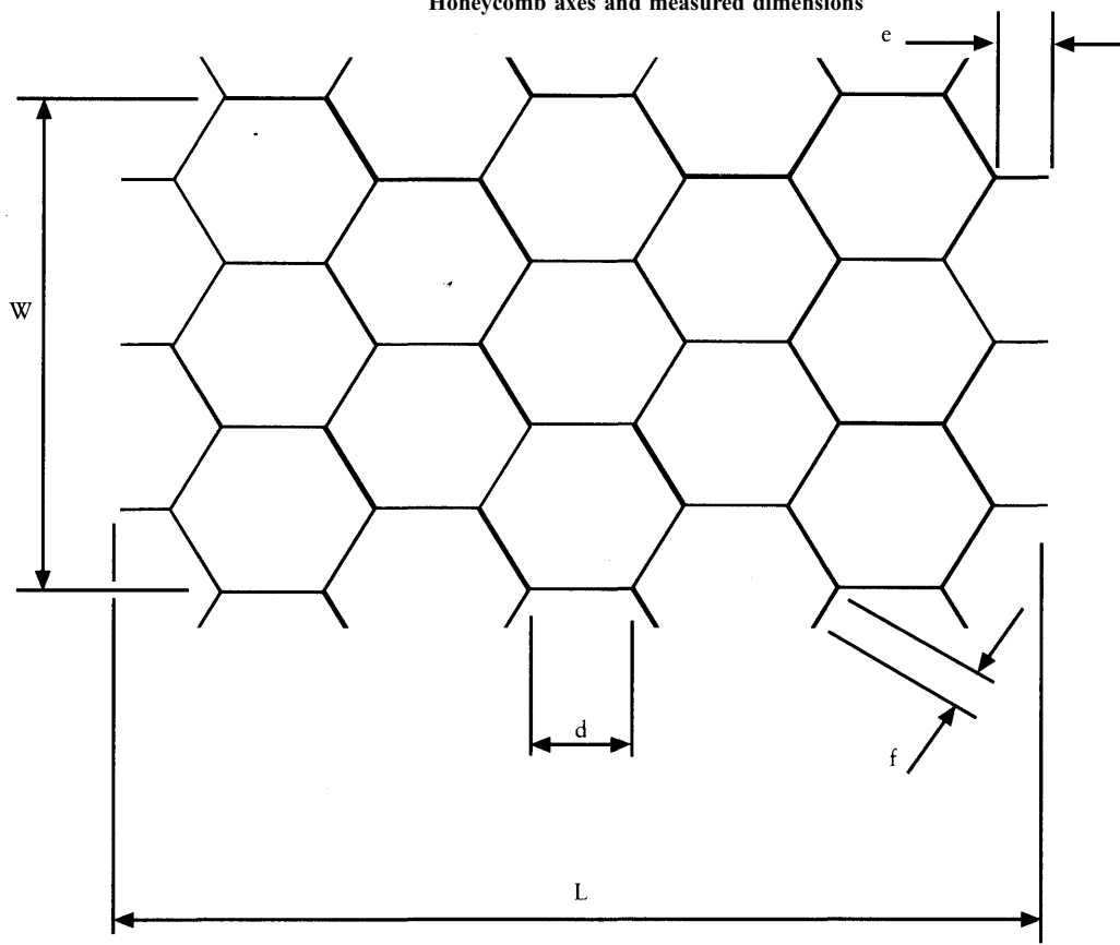
Figure 3 Honeycomb axes and measured dimensions
