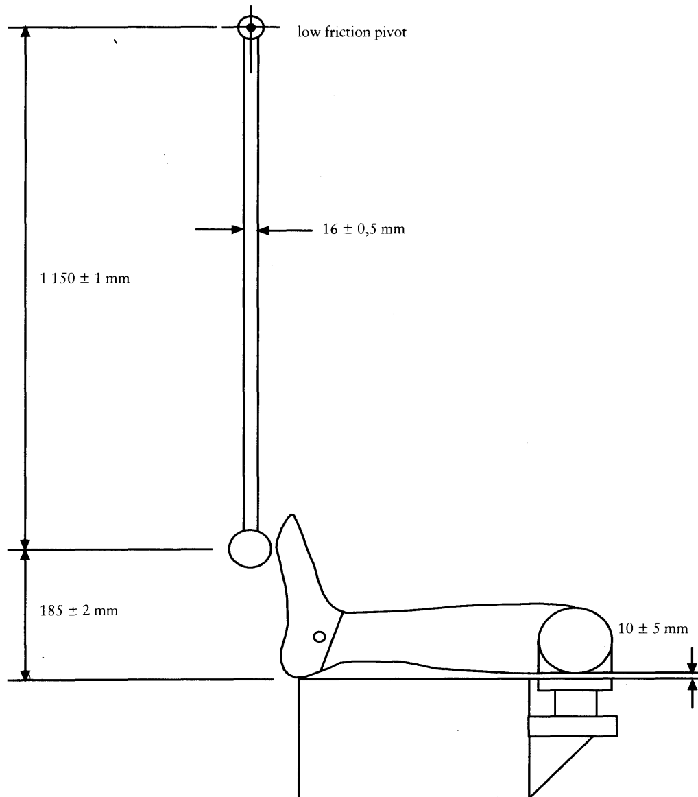
Figure 2 Upper foot impact test — test set-up specifications
