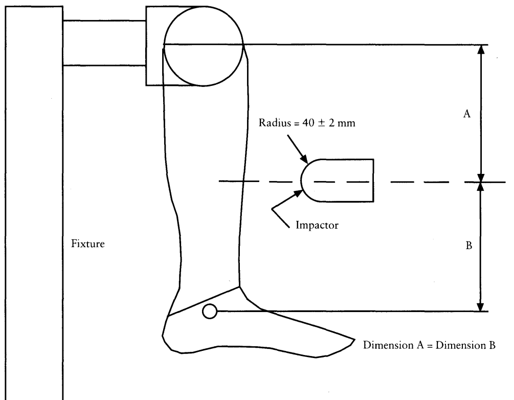
Figure 1 Tibia impact test — test set-up specifications
