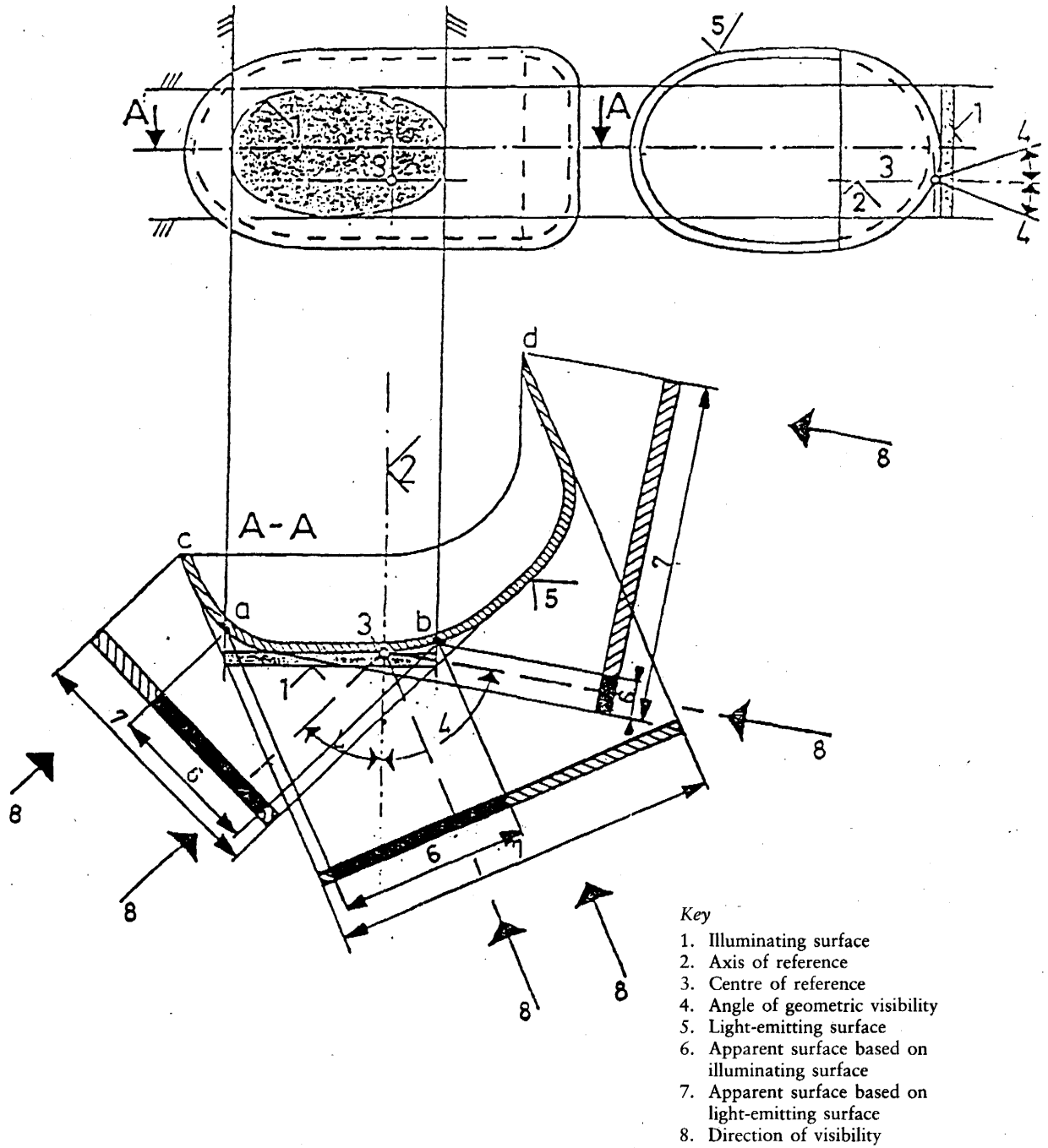
Lamp surfaces, axis and centre of reference, and angles of geometric visibility
