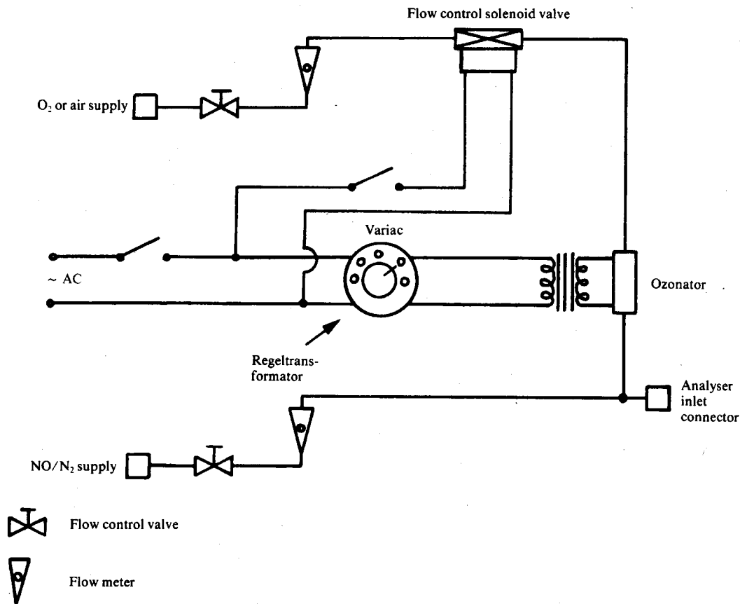
Diagram of NO x converter efficiency device
