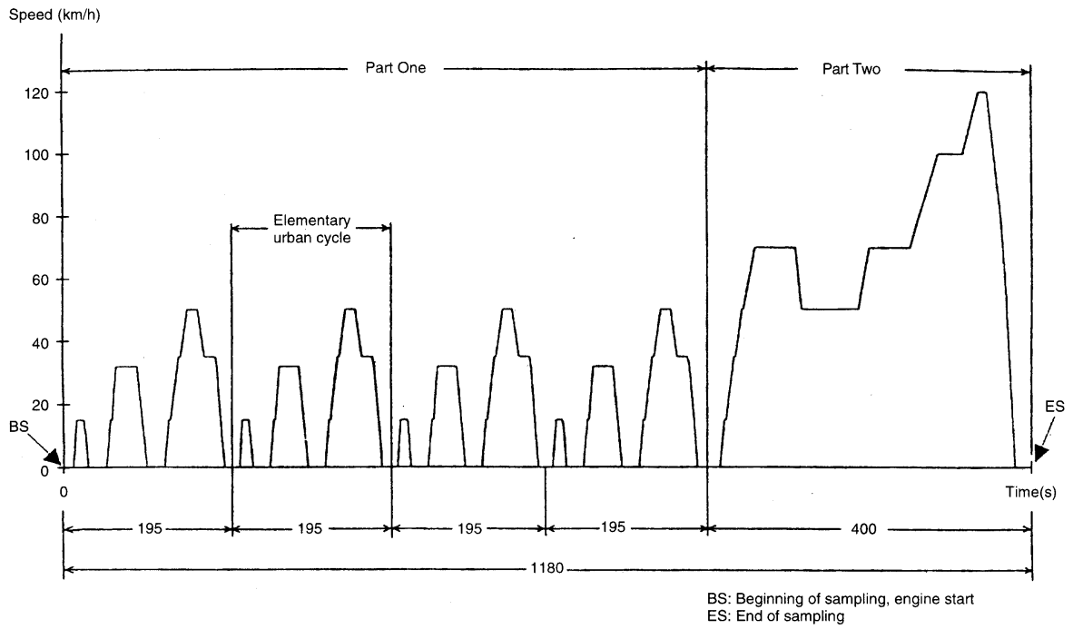
Figure III.1.1 Operating cycle for the Type I test
