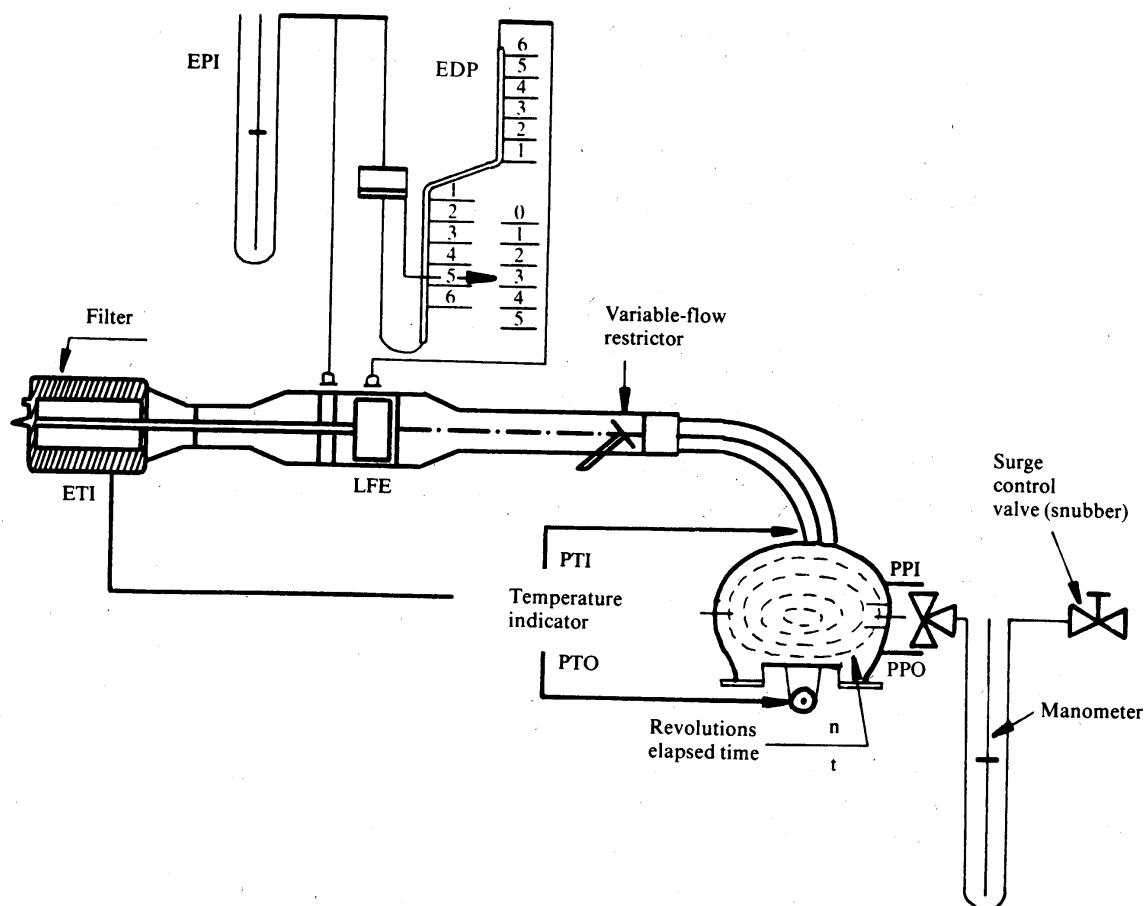
Figure III.6.4.2.3.1 PDP-CVS calibration configuration
