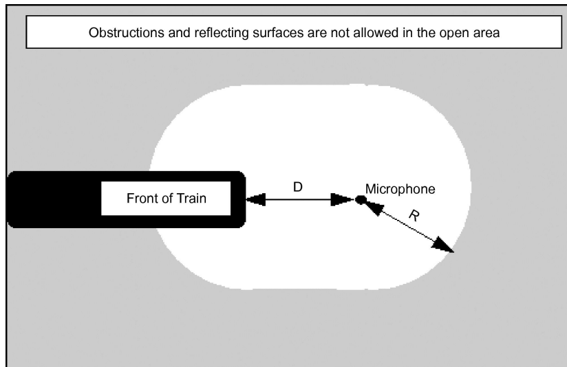
Open site for warning horn measurements
