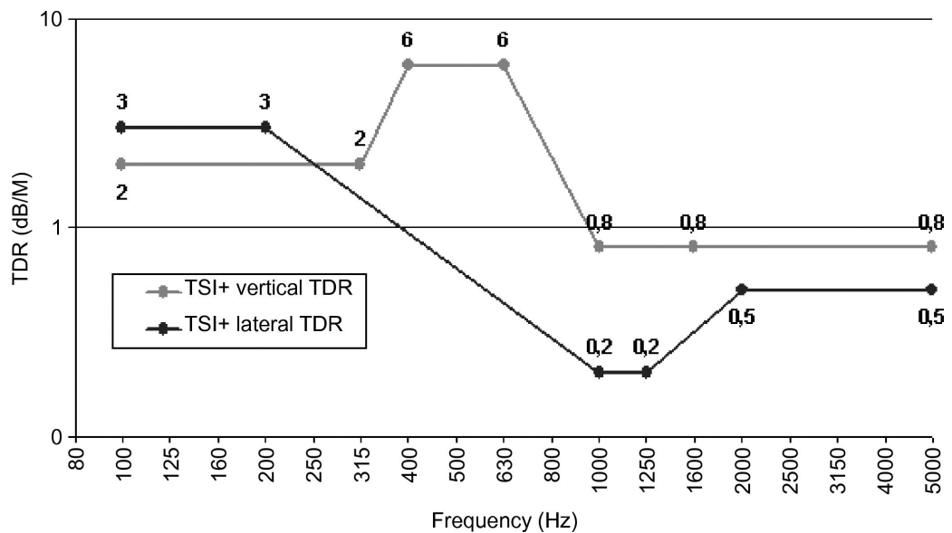
Vertical and lateral decay rate lower limit spectrum of the reference track
