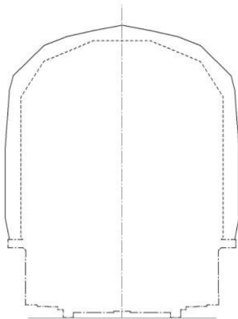
UK1 (issue 2) profiles
