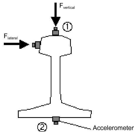
Figure N3 captor location on the rail cross section
