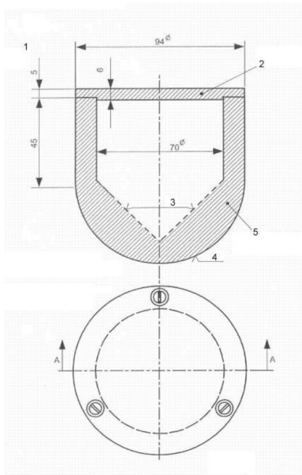
Figure J.2 Diagram of projectile
