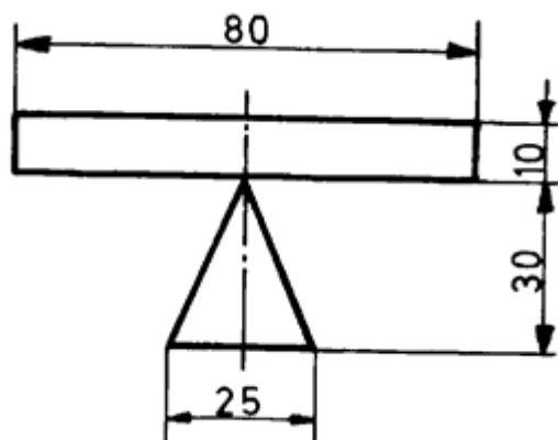
Fig. B19 Lifting at 4 points with or without running gear.
