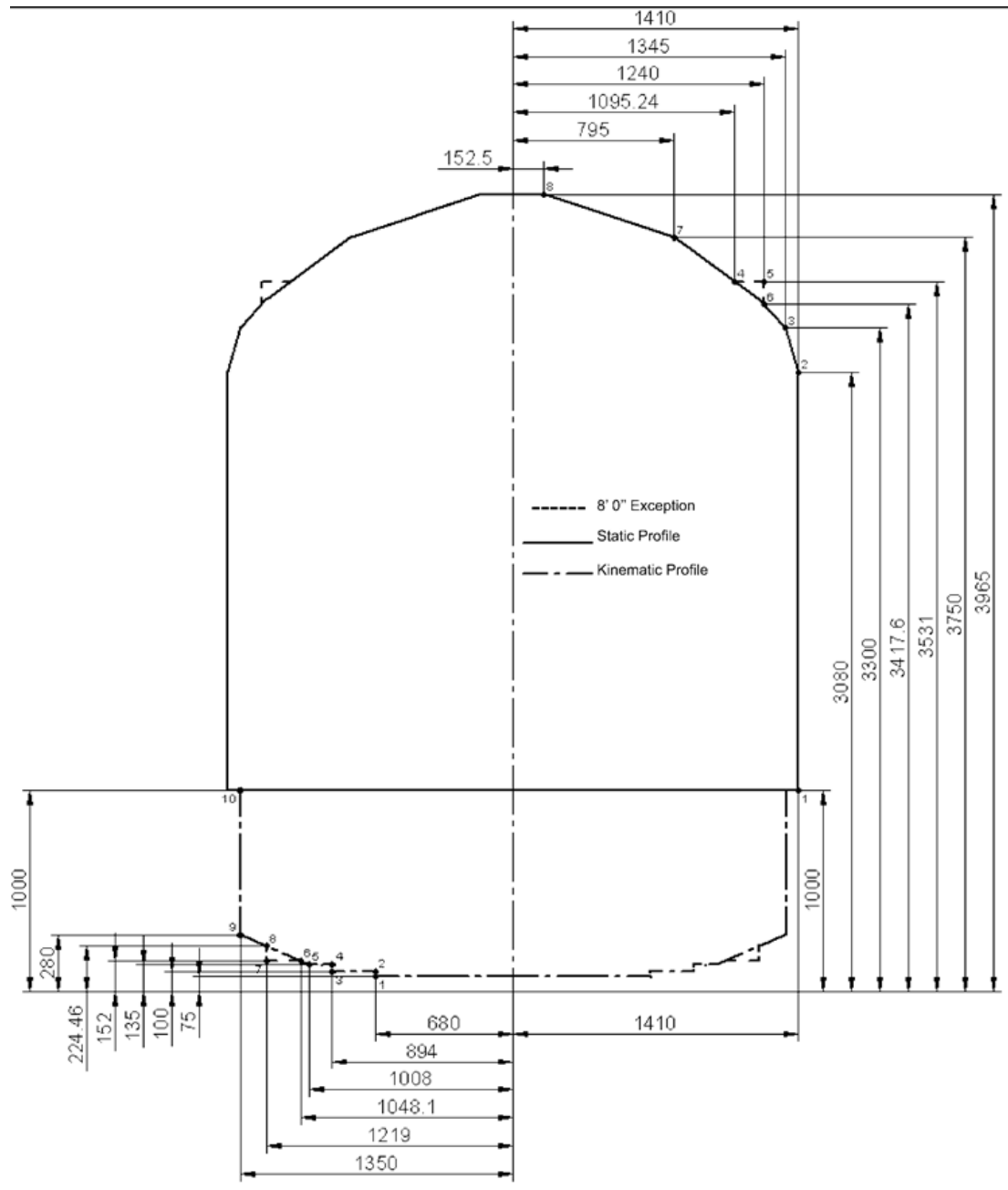
Fig. U6 Lower parts for kinematic gauge WM-02, 1, 0
