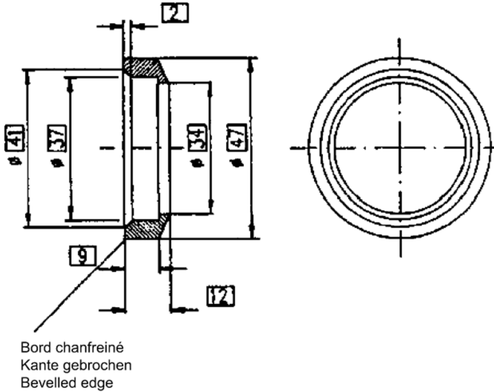
Fig. I.14 Coupling Head — Main Reservoir Pipe
