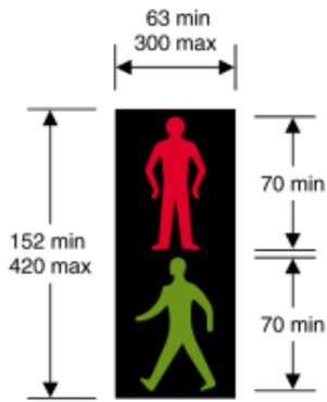
4003.1A Supplementary near side light signals for pedestrians at a pedestrian facility controlled by light signals
