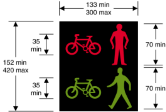
4003.7A Supplementary near side light signals for pedestrians and cyclists at a Toucan crossing
