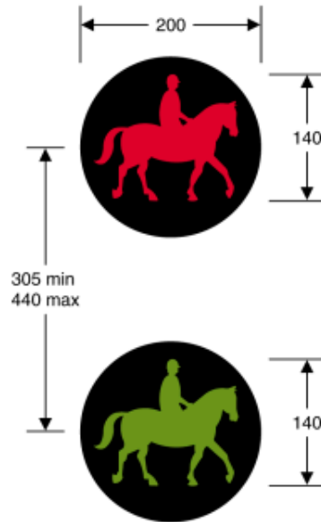
4003.2 Light signals for equestrian traffic
