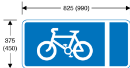
959.1 With-flow cycle lane
