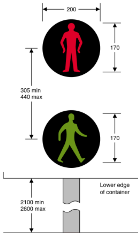
4002.1 Light signals for pedestrians
