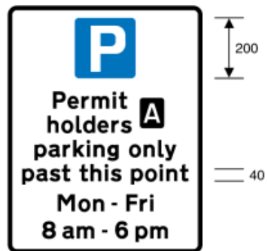
663.3 Entrance to a road or area where parking is reserved for permit holders during the period indicated and where parking bays have not been provided
