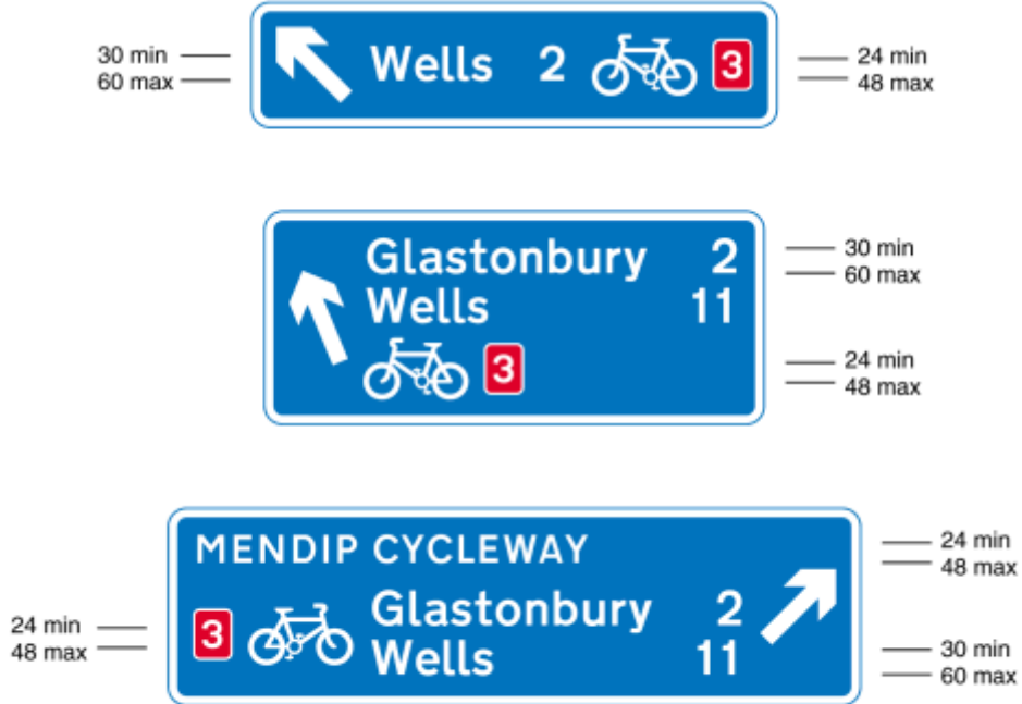
2602.1A Same as diagram 2602.1 (Alternative types)
