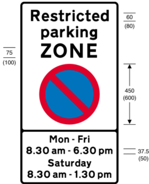
663.2 Entrance to a restricted parking zone
