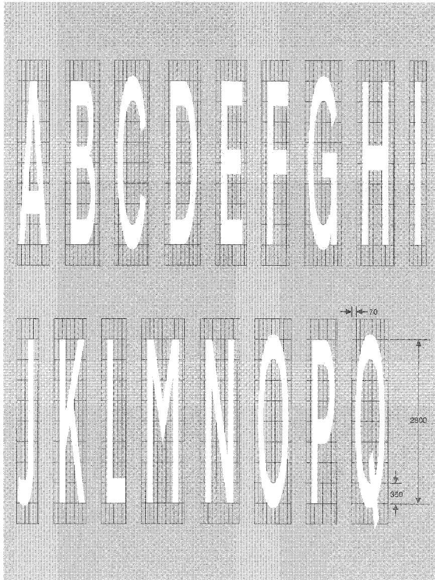
SCHEDULE 13 PART VI Regulation 13(6) PROPORTIONS AND FORM OF LETTERS, NUMERALS AND OTHER CHARACTERS FOR USE IN THE ROAD MARKINGS SHOWN IN SCHEDULE 6 (b) with a height of 2.8 metres
