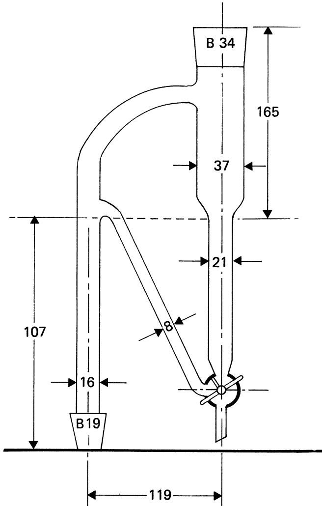
DIAGRAM OF A MODIFIED CLEVINGER-TYPE SEPARATOR
