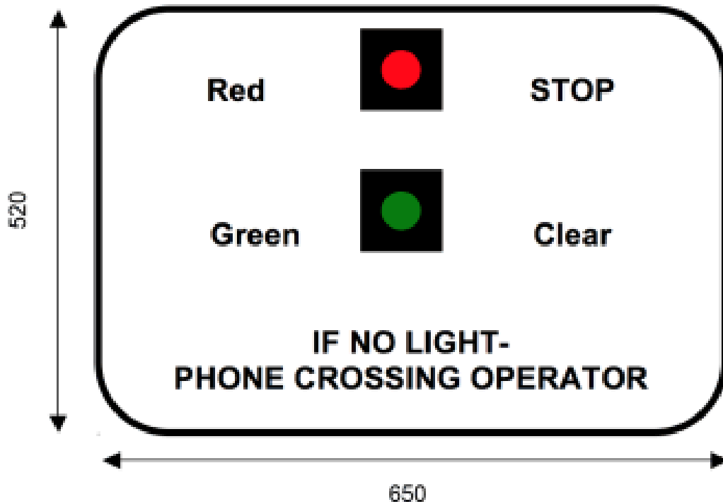
Black lettering and border on white background Sign for use with miniature stop lights at a crossing with a telephone
