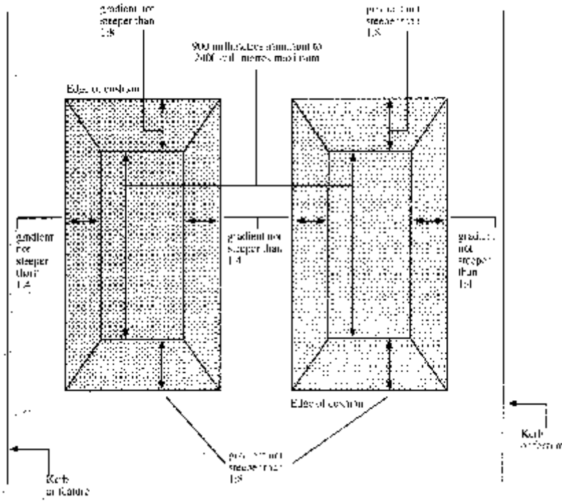
Diagram 5a. Cushion Type Hump Plan View
