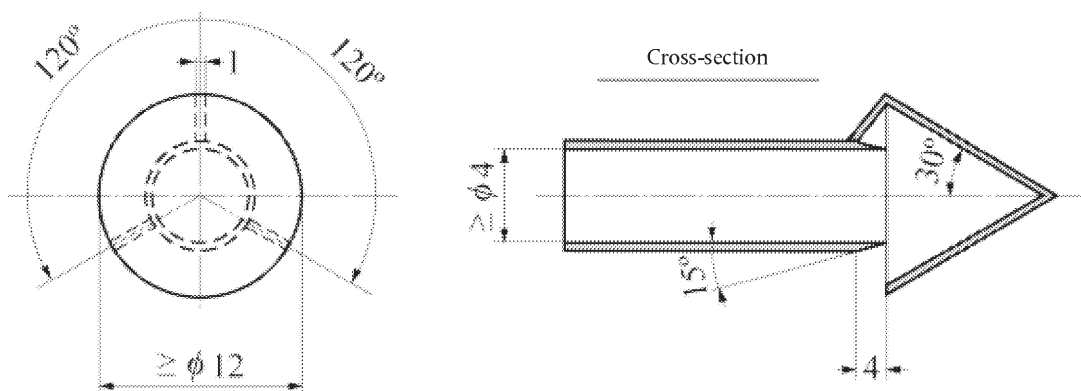
Scheme of a sampling probe with a hat-shaped pre-classifier
