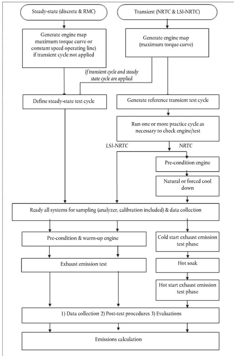
Figure 6.4 Test sequence
