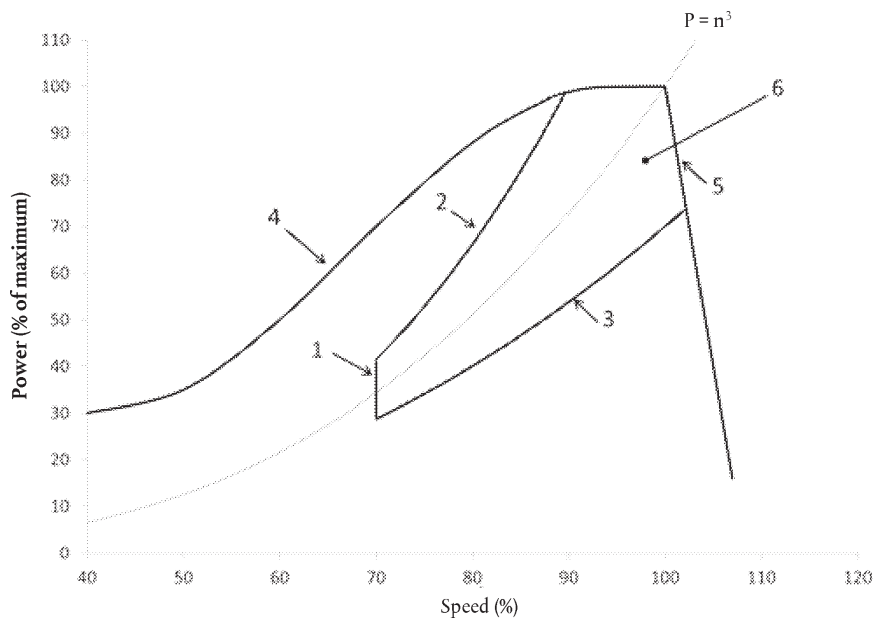
Control area for engines tested on NRSC cycle E3
