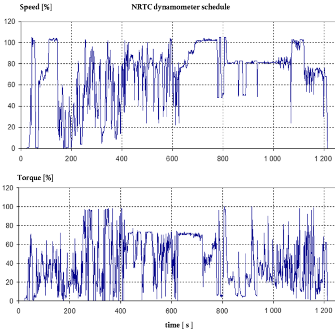
Figure 6.3 NRTC normalized dynamometer schedule
