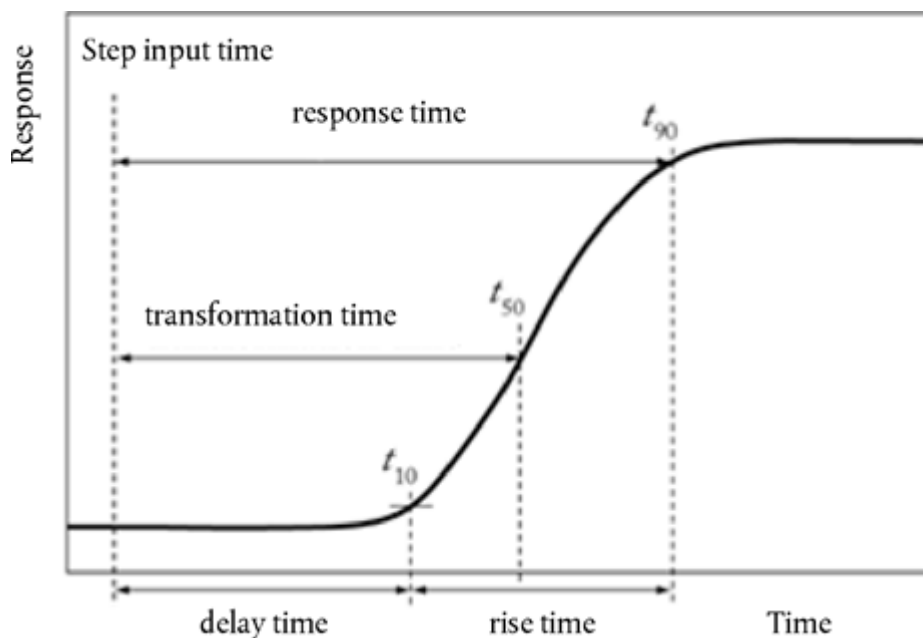
[ F1 Figure Illustration of system responses] 6-11
