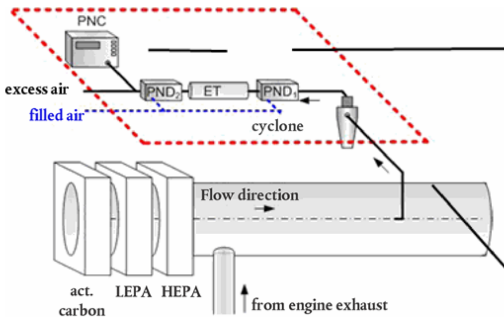
f1 Figure Schematic of recommended particle sampling system – Full flow sampling] 6.10
