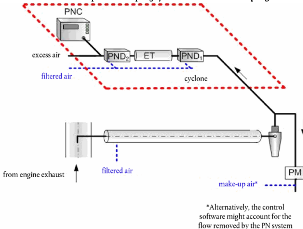
f1 Figure Schematic of recommended particle sampling system – Full flow sampling] 6.10
