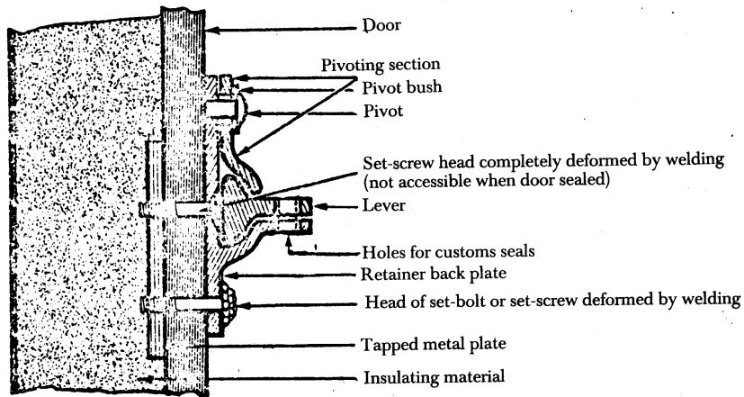
Customs sealing device
