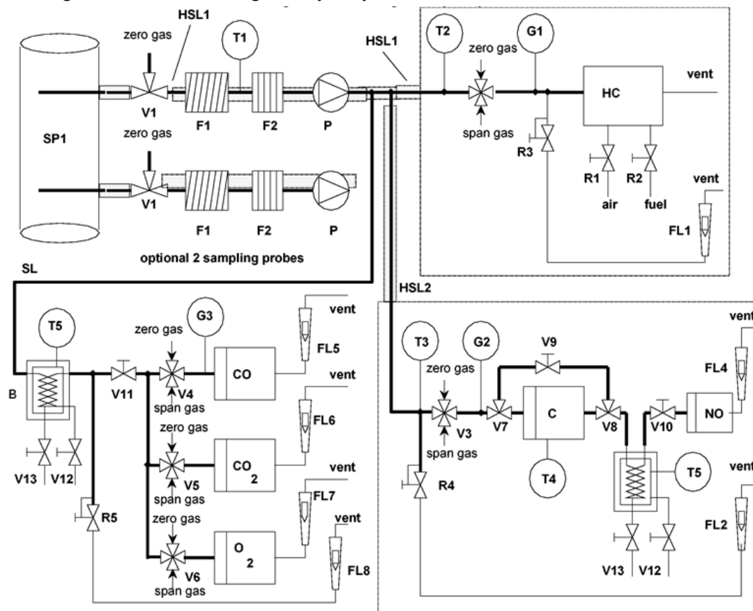
Flow diagram of dilute exhaust gas analysis system for CO, CO 2 , NO x and HC
