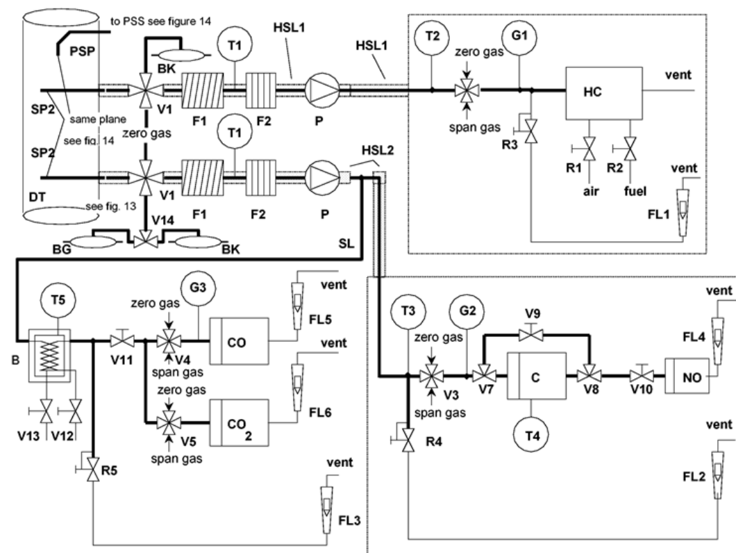
Partial flow dilution system with isokinetic probe and fractional sampling (SB control)
