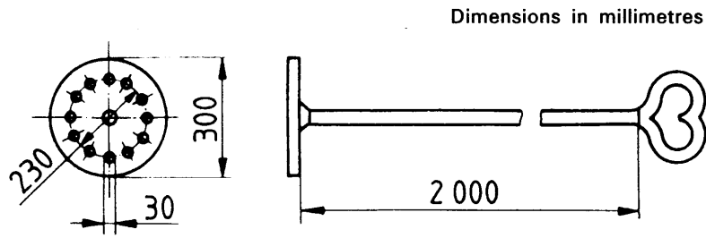
Figure 2: Suitable plunger for small tanks
