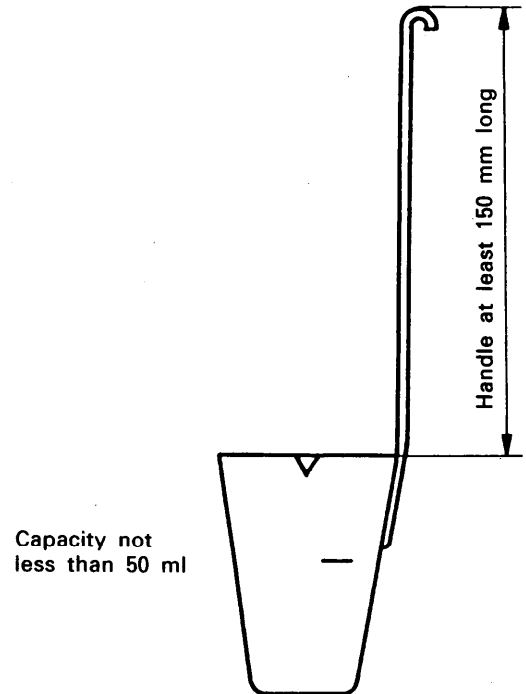
Figure 4: Suitable dipper for liquids
